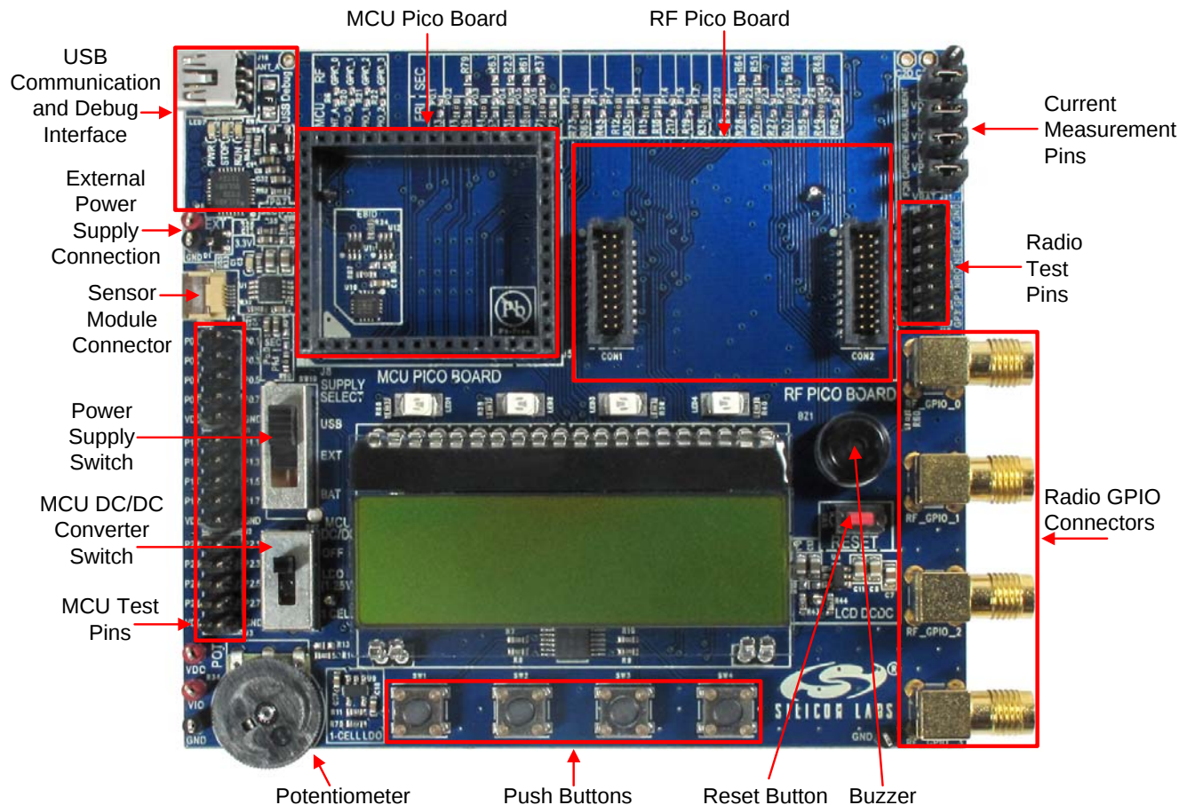
Figure 3. Wireless Motherboard
