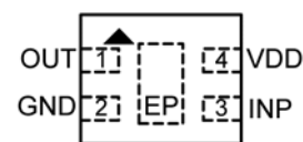
MIC842 4-Pin 1.2mm × 1.6mm TDFN (MT) (Top View)
