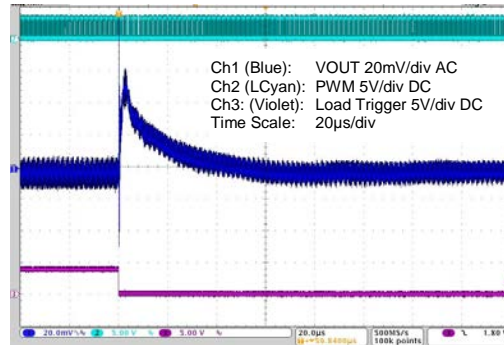
Figure 5.40 20 to 5A Load Step – Max. Capacitance
