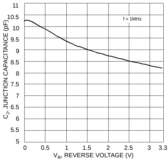
Figure 5 Typical Capacitance
