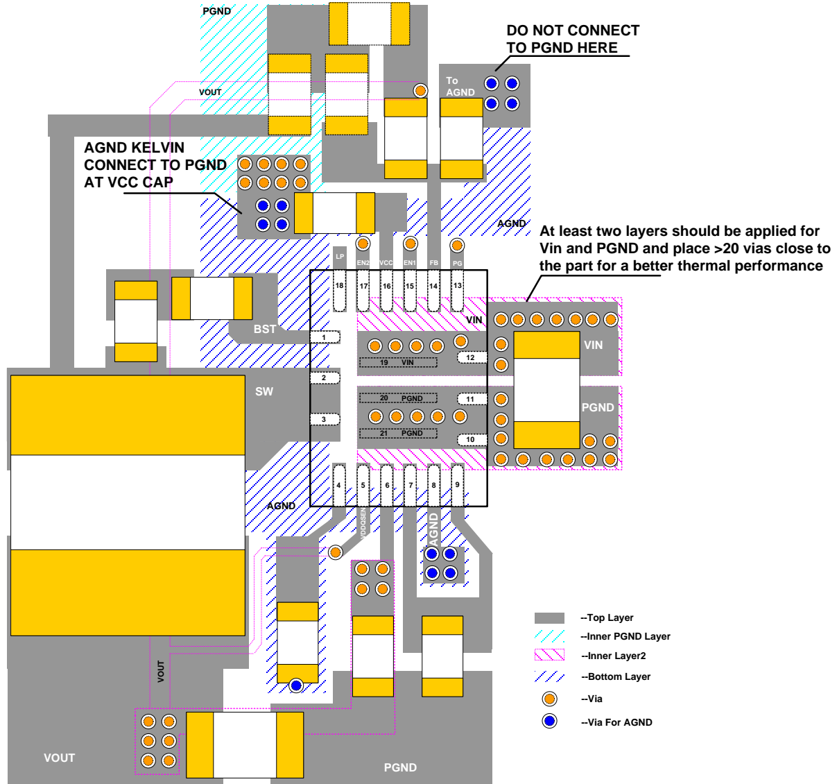
Figure 13—Recommend Layout
