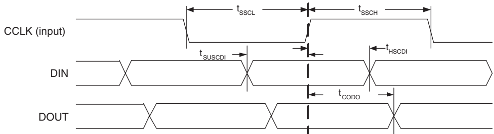
Figure 3-19. sysCONFIG Slave Serial Port Timing
