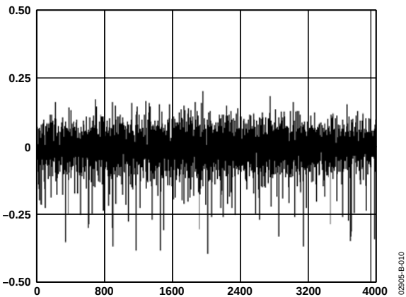
Figure 9. AD9944 Typical DNL Performance
