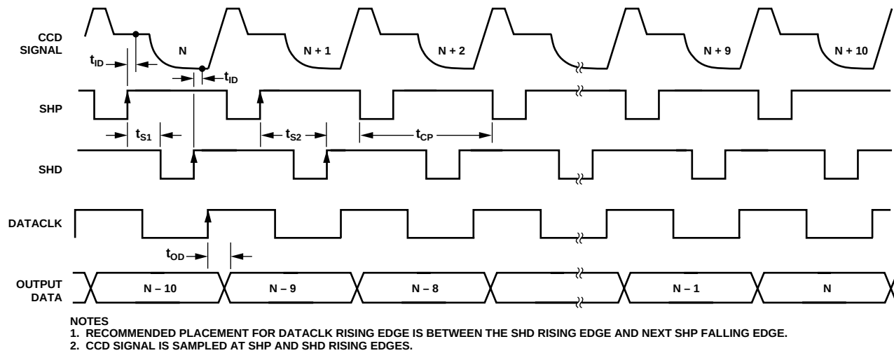
Figure 14. CCD Mode Timing
