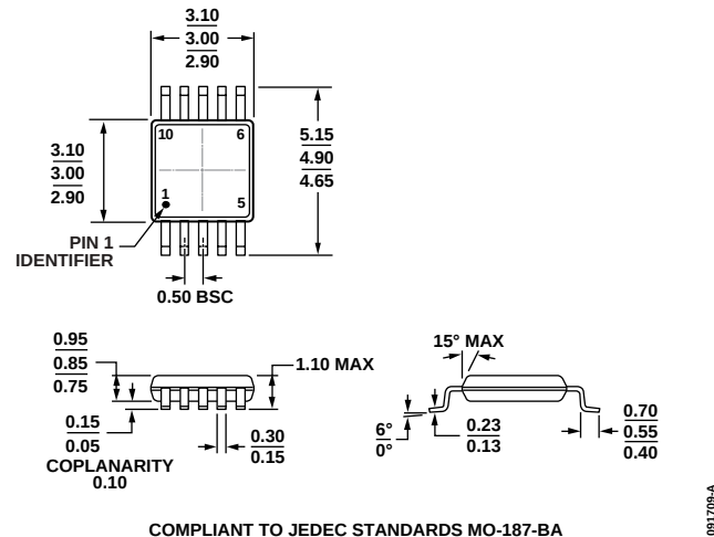
Figure 25. 10-Lead Mini Small Outline Package [MSOP] (RM-10)
