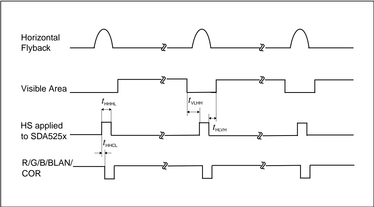
Figure 42 Horizontal Sync-Timing
