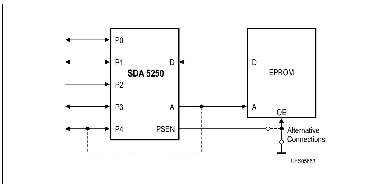
Figure 15 Connecting External Program Memory
