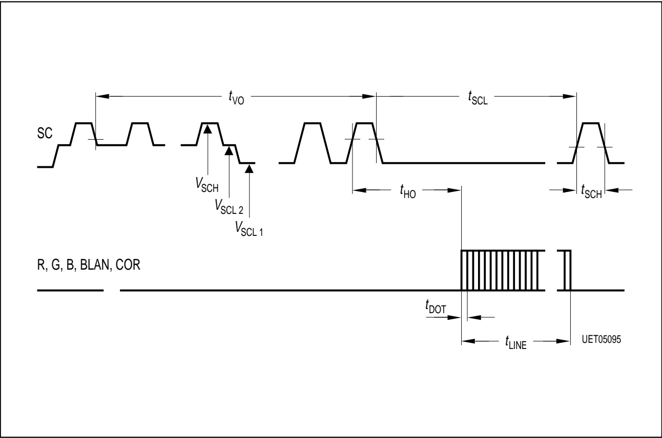
Figure 41 OSD-Input/Output Timing
