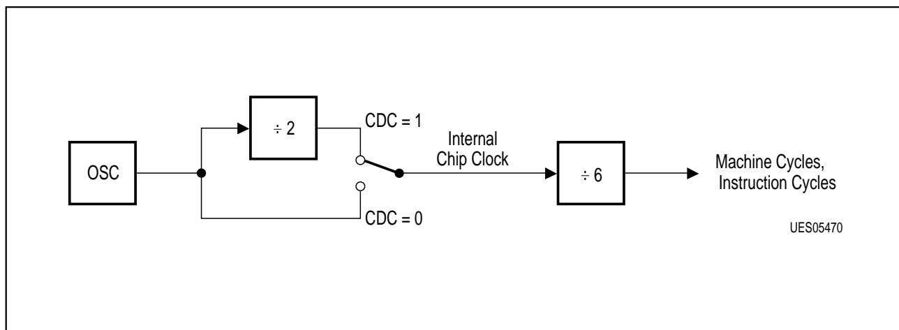
Figure 14 CPU-Timing
