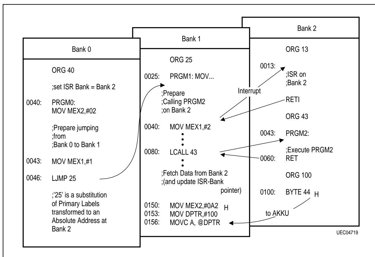
Figure 20 Program Example
