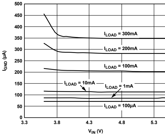
Figure 14. Ground Current vs. Input Voltage
