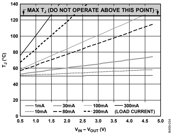
Figure 38. 0 \text{ mm}^2 of PCB Copper, T_A = 50^{\circ}\text{C}
