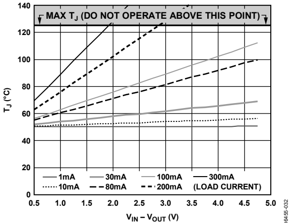
Figure 36. 500 \text{ mm}^2 of PCB Copper, T_A = 50^{\circ}\text{C}
