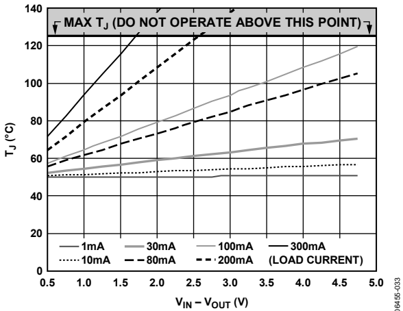
Figure 37. 100 \text{ mm}^2 of PCB Copper, T_A = 50^{\circ}\text{C}
