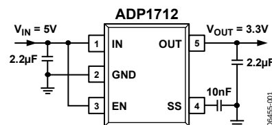
Figure 1. ADP1712 with Fixed Output Voltage and Soft-Start Capacitor, 3.3 V
