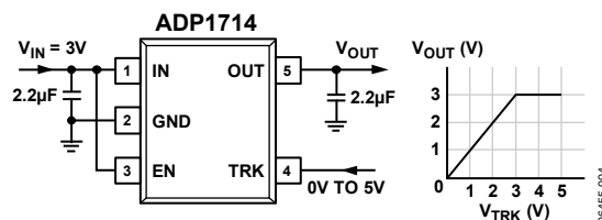
Figure 4. ADP1714 with Output Voltage Tracking
