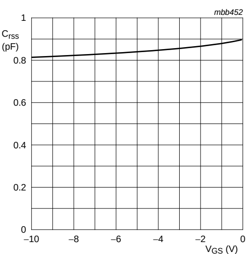
Fig 17. Reverse transfer capacitance as a function of gate-source voltage; typical values.
