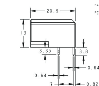
Board Mount Header Assembly
