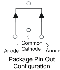
TO-220AB Bottom View
