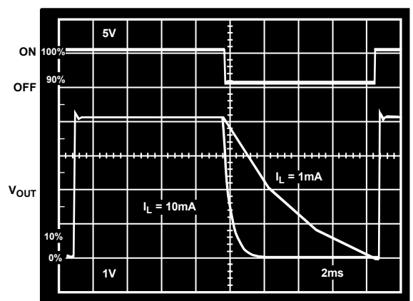
Figure 16. SLEEP Response Time
