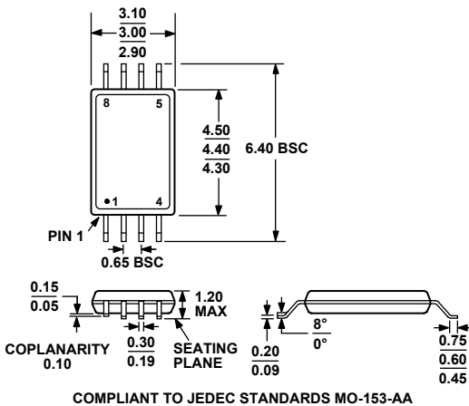
COMPLIANT TO JEDEC STANDARDS MO-153-AA Figure 33. 8-Lead Thin Shrink Small Outline Package [TSSOP] (RU-8) Dimensions shown in millimeters
