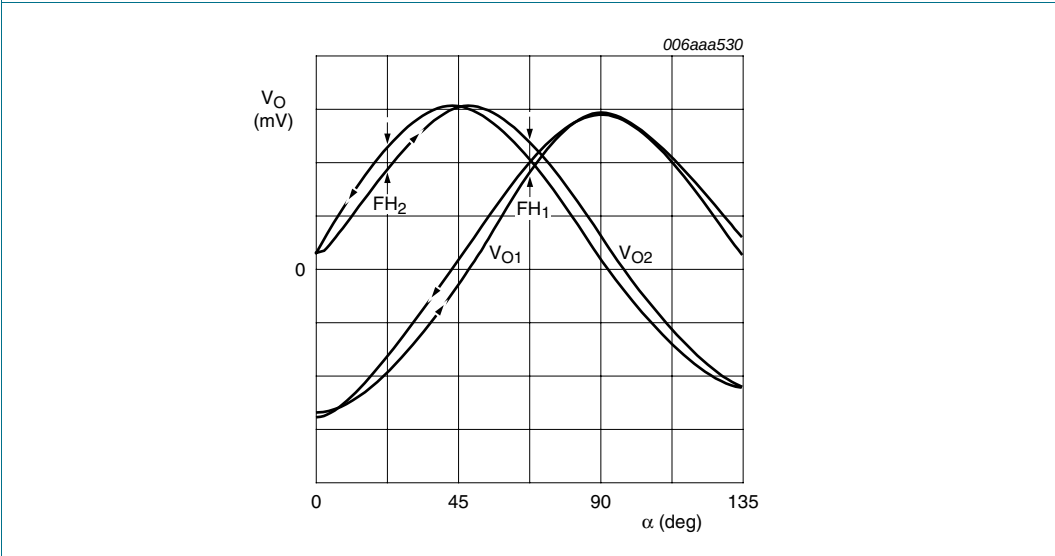
Fig 3. Definition of hysteresis
