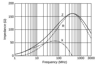
BLM18AG121SN1
