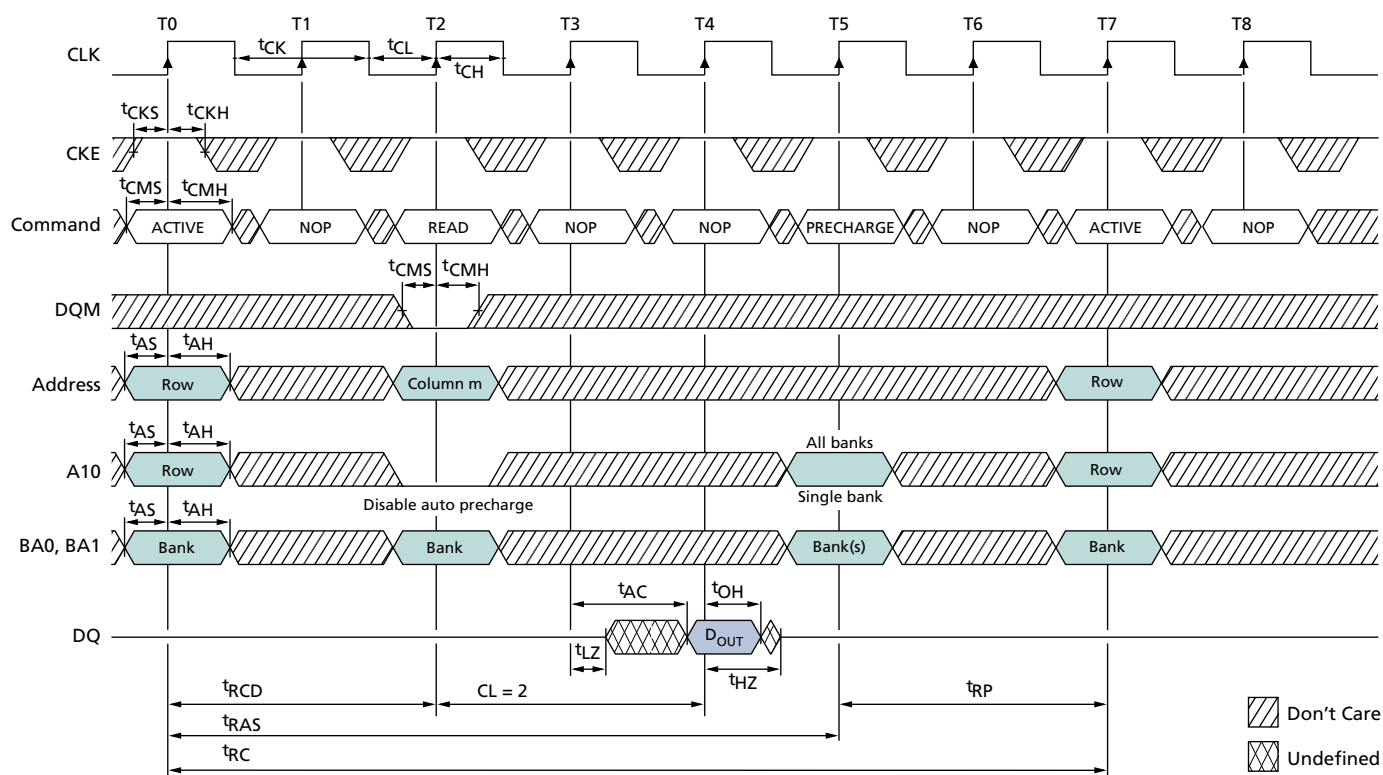
Figure 39: Single READ Without Auto Precharge
