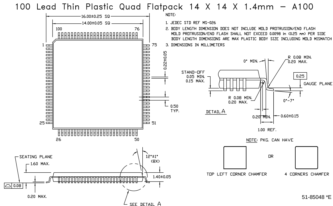
Figure 17. 100-Pin TQFP (14X14X1.4 mm)
