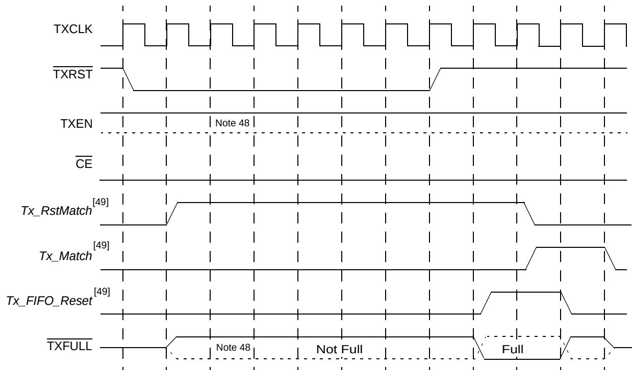
Figure 13. Transmit FIFO Reset Sequence with Constant \overline{\text{CE}}
