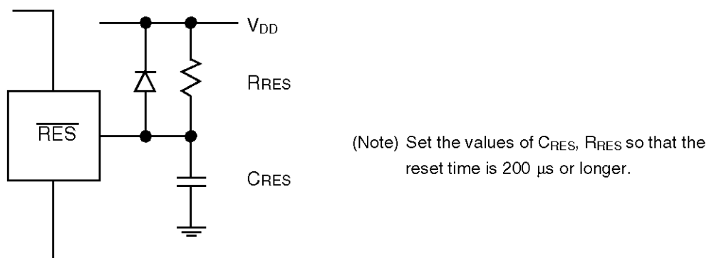
Figure 4 Reset Circuit
