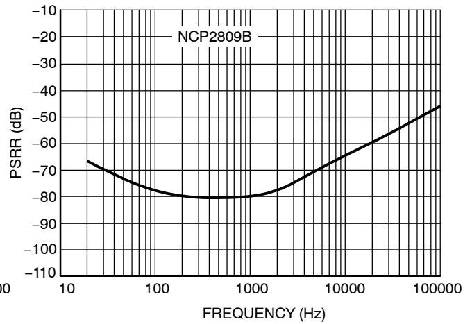
Figure 35. PSRR – Input Grounded with 10\ \Omega V_p = 5.0\ \text{V} , V_{\text{ripple}} = 200\ \text{mV pk-pk} , R_L = 16\ \Omega , G = 1 (0 dB)
