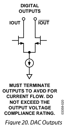
Figure 20. DAC Outputs
