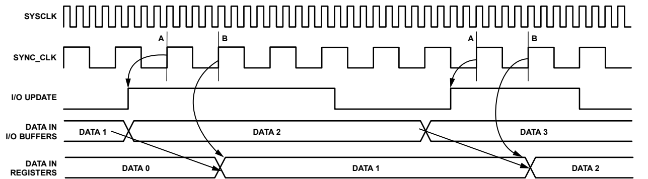
THE DEVICE REGISTERS AN I/O UPDATE AT POINT A. THE DATA IS TRANSFERRED FROM THE I/O BUFFERS AT POINT B.
