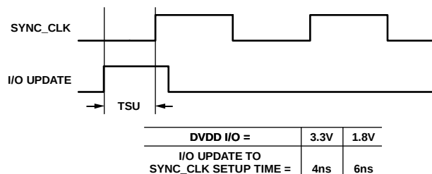
Figure 24. Setup Time for I/O Update Pulse for Synchronous Data Transfer
