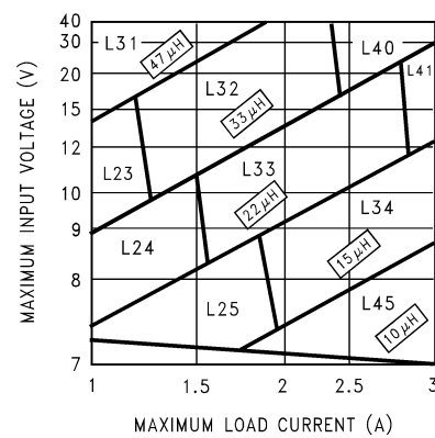
Figure 22. LM2676-5.0
