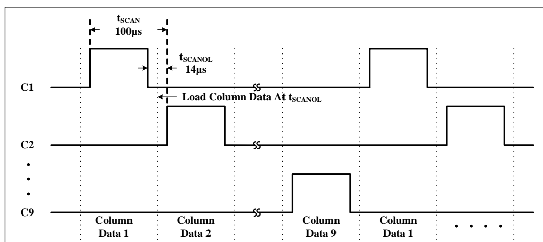
Figure 4 Scanning Timing
