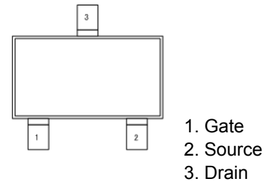
SOT-23(TOP VIEW)
