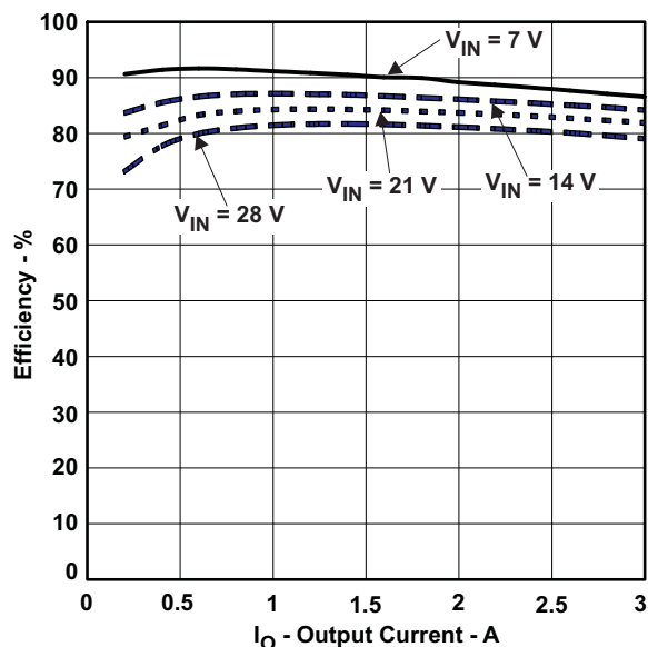
Figure 17. TPS54331D Efficiency
