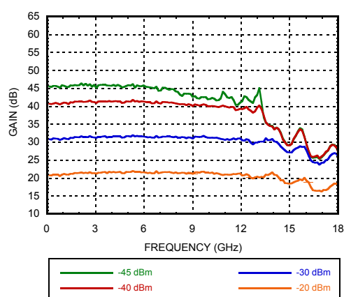
Response vs. Input Power [1][3][5]
