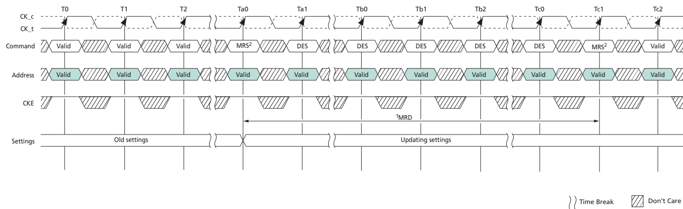
Figure 13: t^{\text{MRD}} Timing
