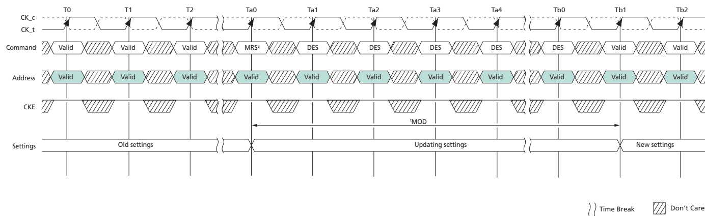
Figure 14: t^{\text{MOD}} Timing
