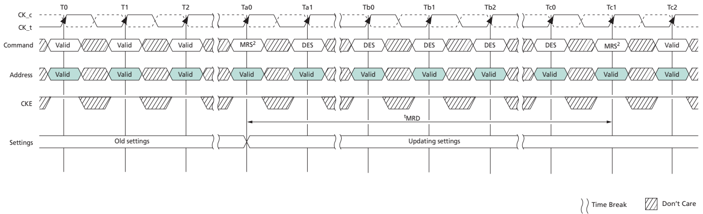
Figure 13: t_{MRD} Timing
