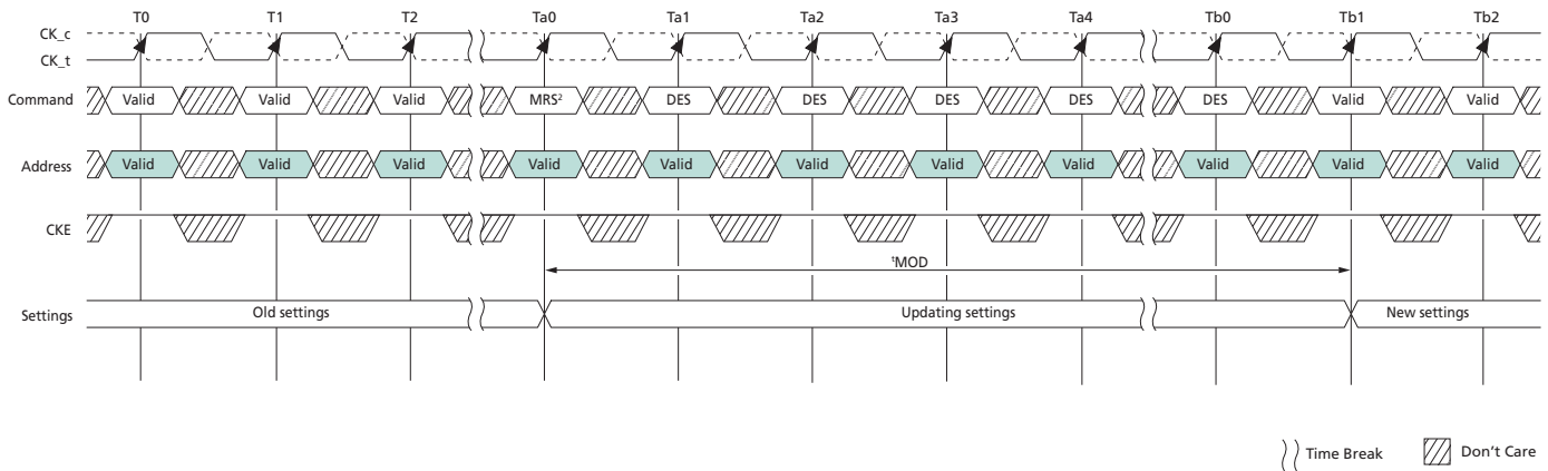
Figure 14: t_{MOD} Timing
