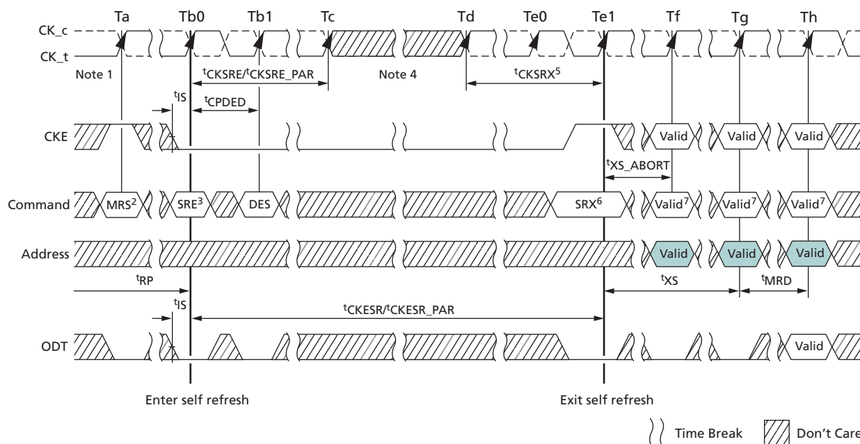
Figure 17: DLL Switch Sequence from DLL-Off to DLL-On
