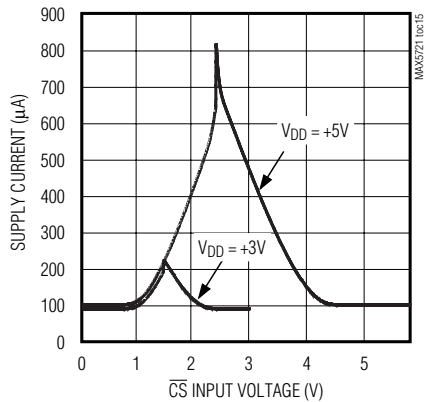
SUPPLY CURRENT vs. CS INPUT VOLTAGE
