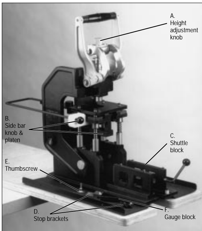
Figure 4. 10960-2000 Hand Press
