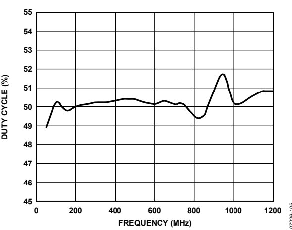
Figure 5. LVDS Output Duty Cycle vs. Frequency
