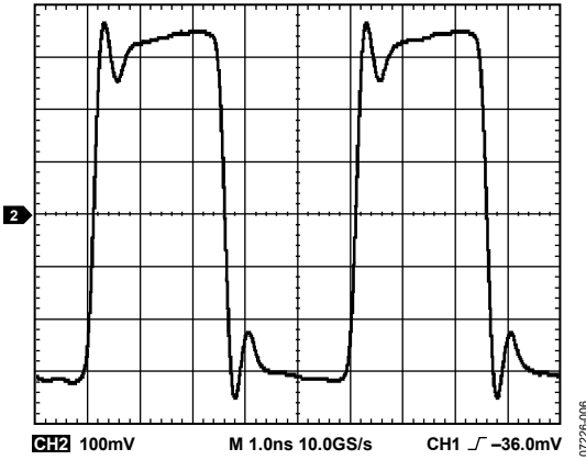
Figure 6. LVDS Output Waveform at 200 MHz
