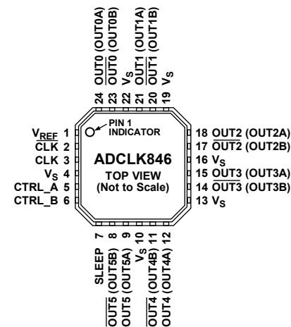
Figure 2. Pin Configuration
