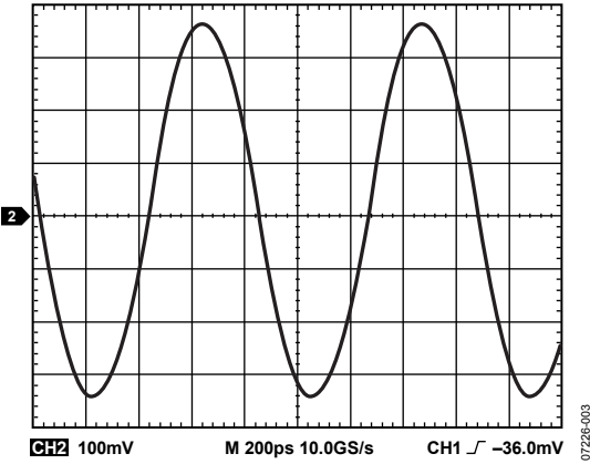
Figure 3. LVDS Output Waveform at 1200 MHz
