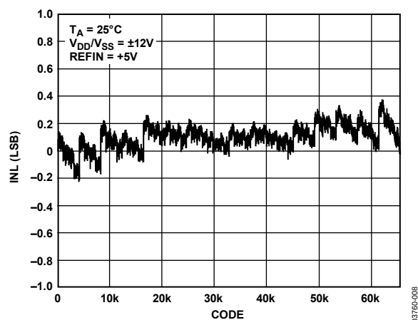
Figure 8. Integral Nonlinearity vs. Code, V_{DD}/V_{SS} = \pm 12\text{ V}
