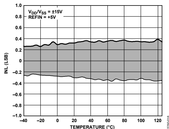
Figure 10. Integral Nonlinearity vs. Temperature, V_{DD}/V_{SS} = \pm 15\text{ V}
