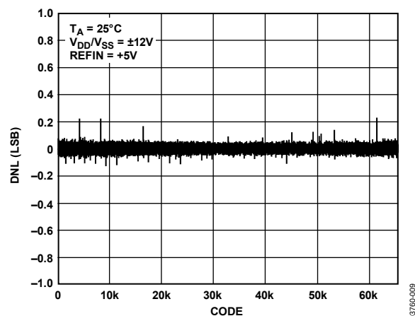
Figure 9. Differential Nonlinearity vs. Code, V_{DD}/V_{SS} = \pm 12\text{ V}
