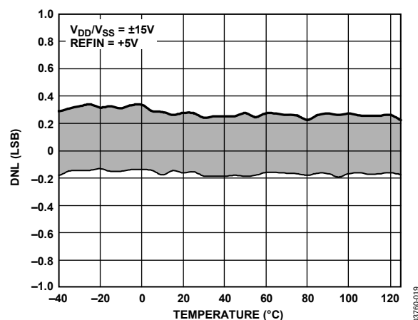
Figure 11. Differential Nonlinearity vs. Temperature, V_{DD}/V_{SS} = \pm 15\text{ V}
