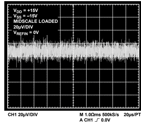
Figure 34. Peak-to-Peak Noise (100 kHz Bandwidth)
