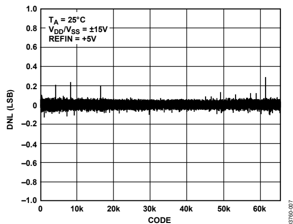
Figure 7. Differential Nonlinearity vs. Code, V_{DD}/V_{SS} = \pm 15\text{ V}
