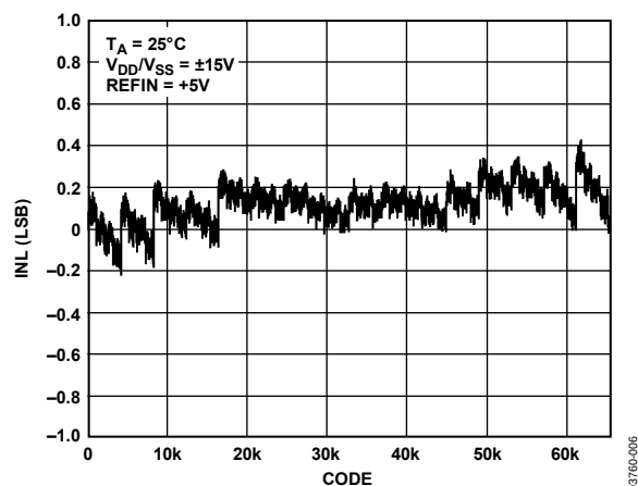
Figure 6. Integral Nonlinearity vs. Code, V_{DD}/V_{SS} = \pm 15\text{ V}
