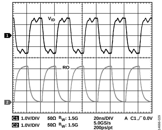
Figure 32. Receiver Propagation Delay at 50 Mbps, |V_{ID}| \geq 1.5 \text{ V}
