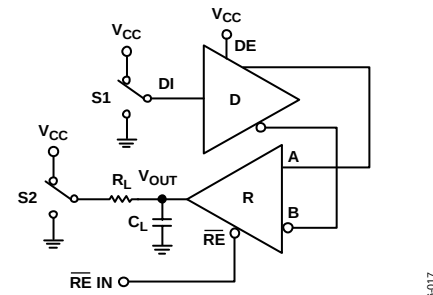
Figure 43. Receiver Enable/Disable from Shutdown
