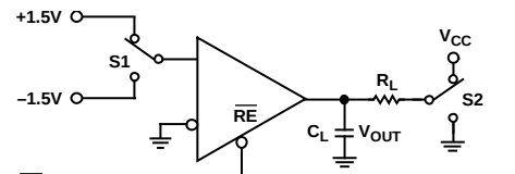
Figure 42. Receiver Propagation Delay/Skew
