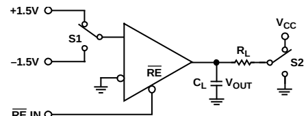
Figure 42. Receiver Propagation Delay/Skew
