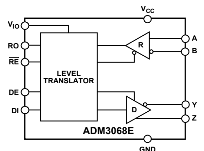
Figure 4. ADM3068E Functional Block Diagram
