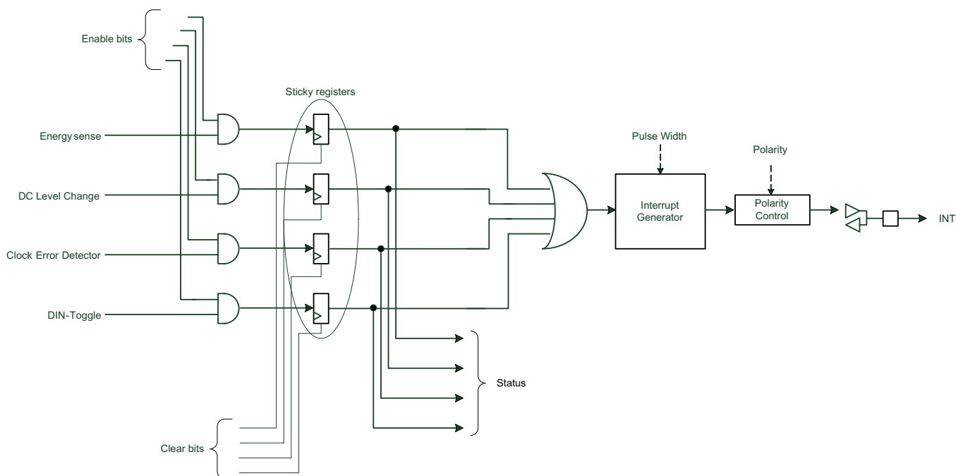
Figure 43. Interrupt Logic
