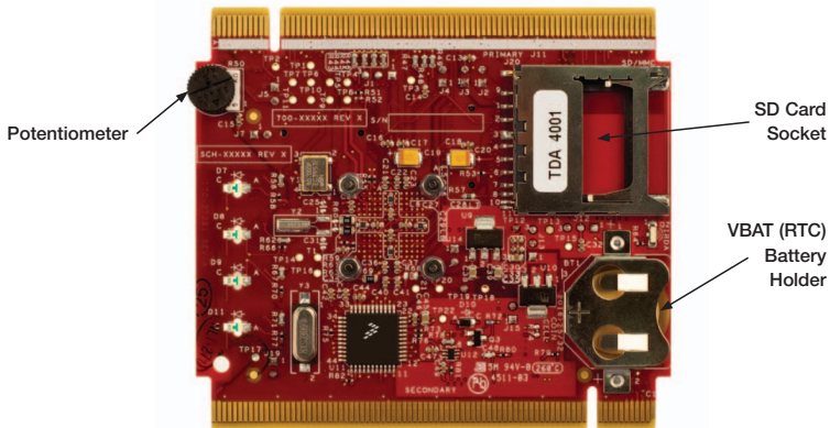
Figure 2: Back side of TWR-K60D100M module.
