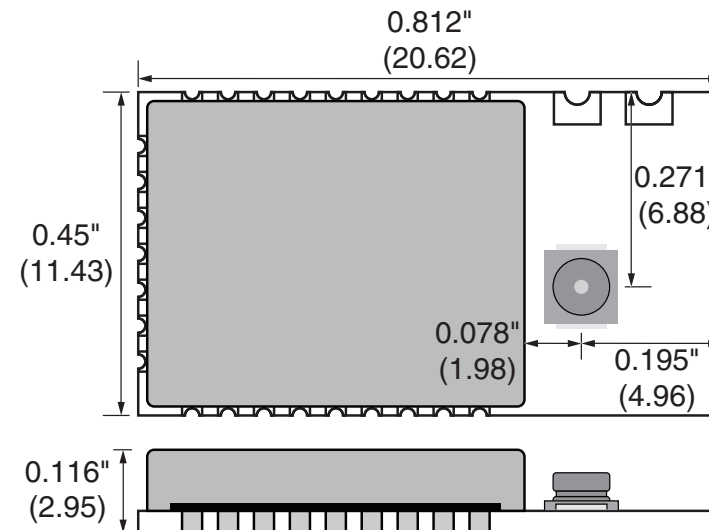
Figure 18: HumPRC™ Series Transceiver Encapsulated Version Dimensions
