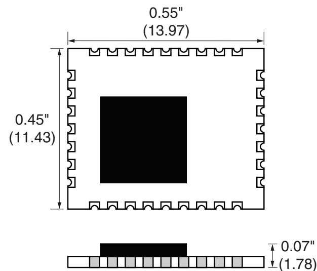
Figure 17: HumPRC™ Series Transceiver Dimensions
