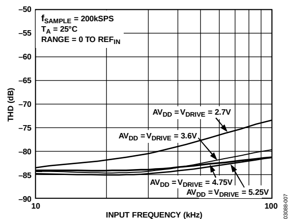
Figure 7. THD vs. Analog Input Frequency for Various Supply Voltages at 200 kSPS
