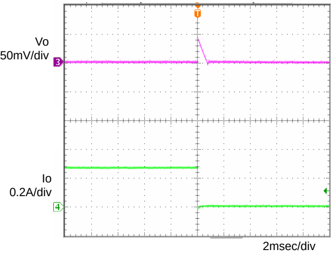
Fig.6 Transient Response (0.3→0A) Co=1 \mu F, Ta=-40°C
