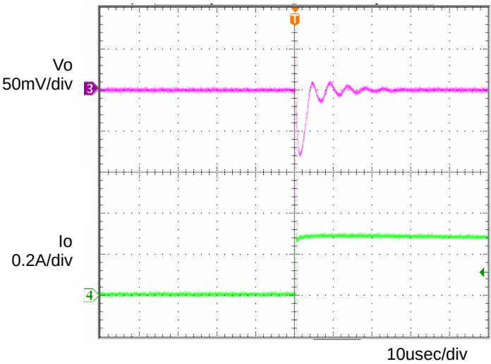
Fig.5 Transient Response (0→0.3A) Co=1 \mu F, Ta=105°C
