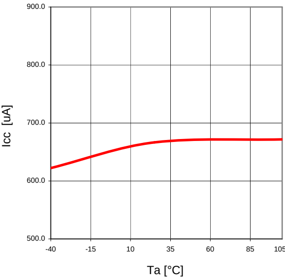
Fig.22 T_a - I_{cc}
