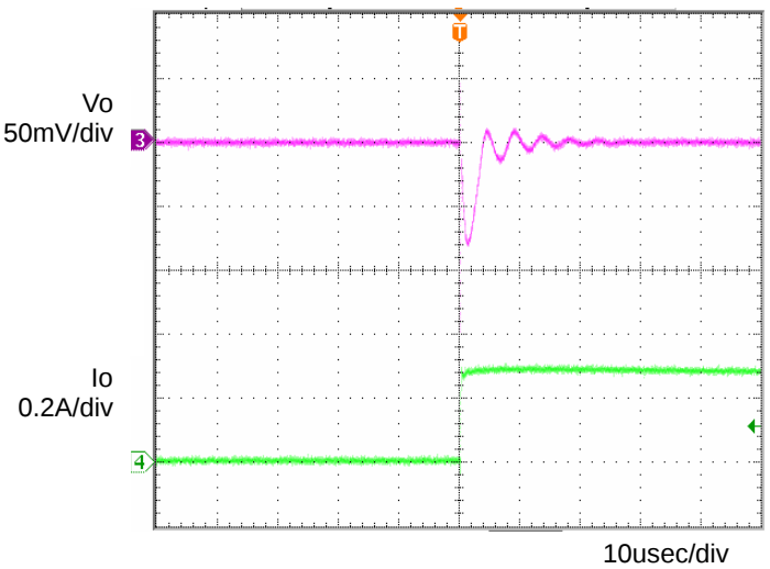
Fig.5 Transient Response (0→0.3A) Co=1 \mu F, Ta=105°C
