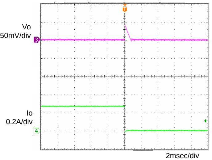
Fig.6 Transient Response (0.3→0A) Co=1 \mu F, Ta=-40°C
