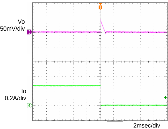
Fig.6 Transient Response (0.3→0A) Co=1μF, Ta=-40°C
