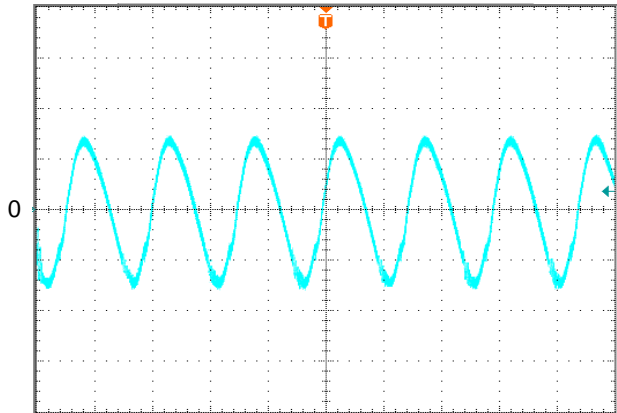
Figure 12: Output voltage ripple at nominal input voltage ( V_{in}=48\text{V} ) and rated load current ( I_o=9\text{A} ) ( 20\text{mV/div} , 2\mu\text{s/div} ). Load capacitance: 1\ \mu\text{F} ceramic capacitor and 10\ \mu\text{F} tantalum capacitor. Bandwidth: 20 MHz. Scope measurements should be made using a BNC cable (length shorter than 20 inches). Position the load between 51 mm to 76 mm (2 inches to 3 inches) from the module
