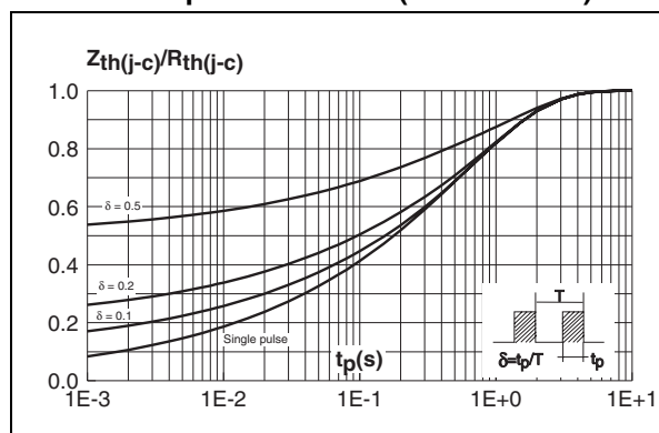
Figure 9. Relative variation of thermal impedance junction to case versus pulse duration (TO-220FPAC)
