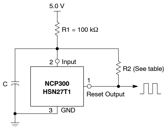
Figure 31. Simple Clock Oscillator
